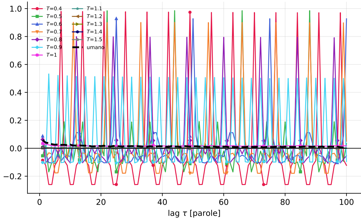
ACF a lag corti — Qwen3.5-4B-Base (cfr. [F] Fig. 5-6)
